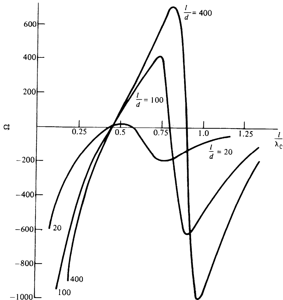
Input reactance of a dipole antenna
