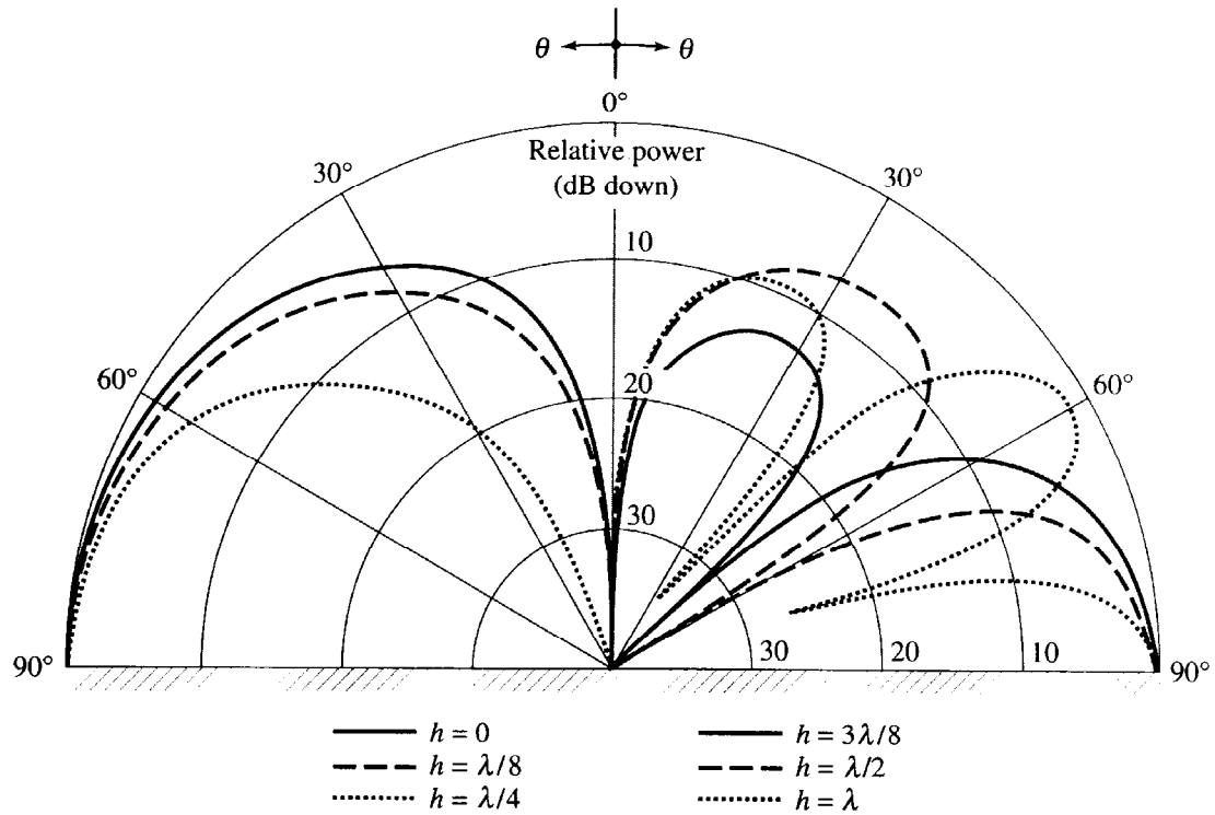
Elevation plane patterns of a vertical infinitesimal electric dipole for different height above a perfectly conducting plane.
