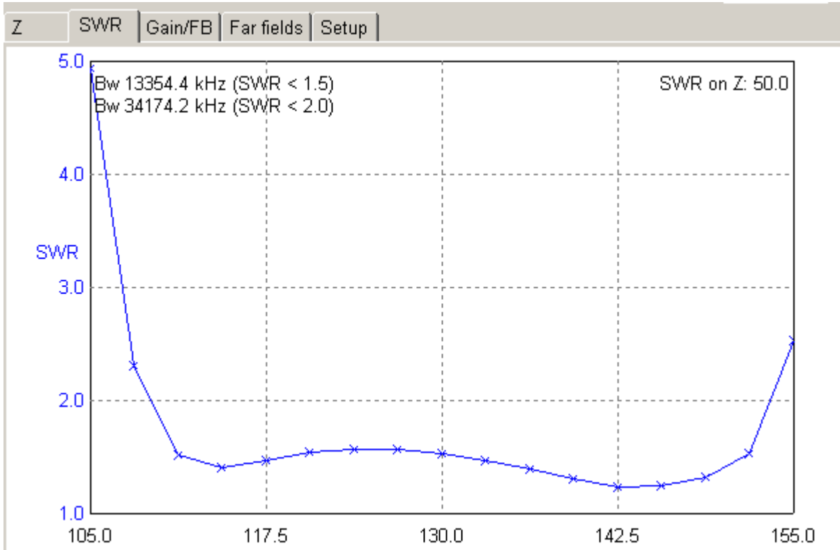
SWR of the 4 Elements Directional Avia Antenna
