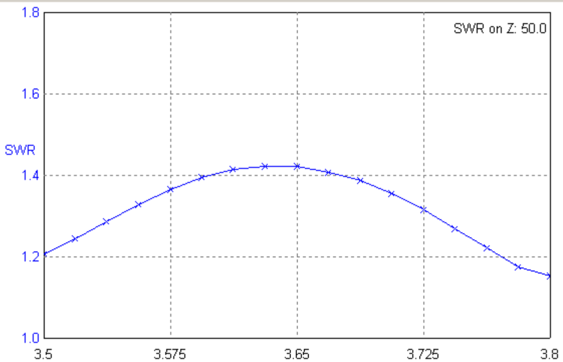
Figure 3 SWR of the DEWD Dipole for the 80- meters with a Stub Matching (30- m above the real ground)
