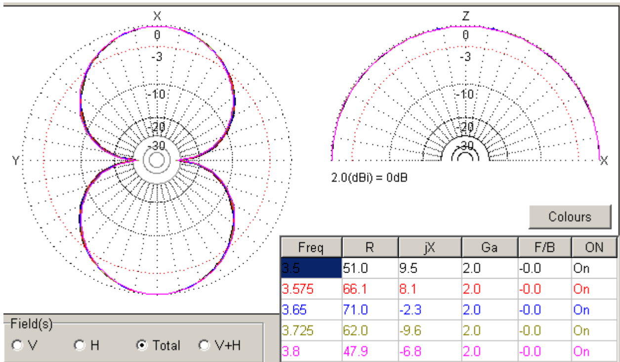
Figure 4 DD of the DEWD Dipole for the 80- meters with a Stub Matching (30- m above the real ground)
