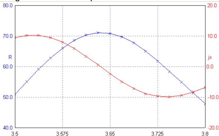
Figure 1 Design of the DEWD Dipole for the 80- meters with Stub Matching
