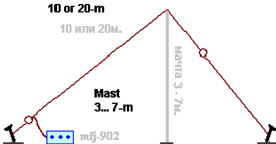
Figure 4 Asymmetrical Dipole Antenna with the End Fed
