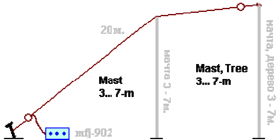
Figure 2 Expedition Antenna Sloper 20- meters length
