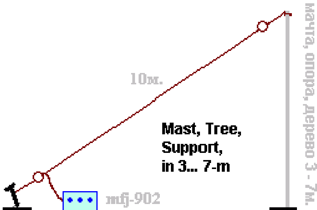
Figure 1 Expedition Antenna Sloper 10- meters length
