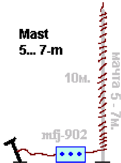
Figure 6 Helical Vertical Antenna
