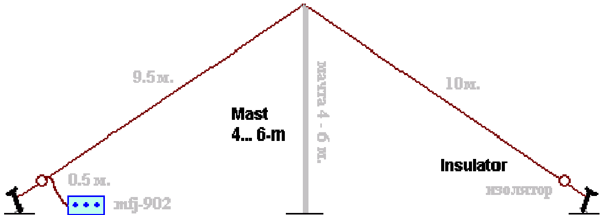
Figure 5 Symmetrical Dipole Antenna with the End Fed
