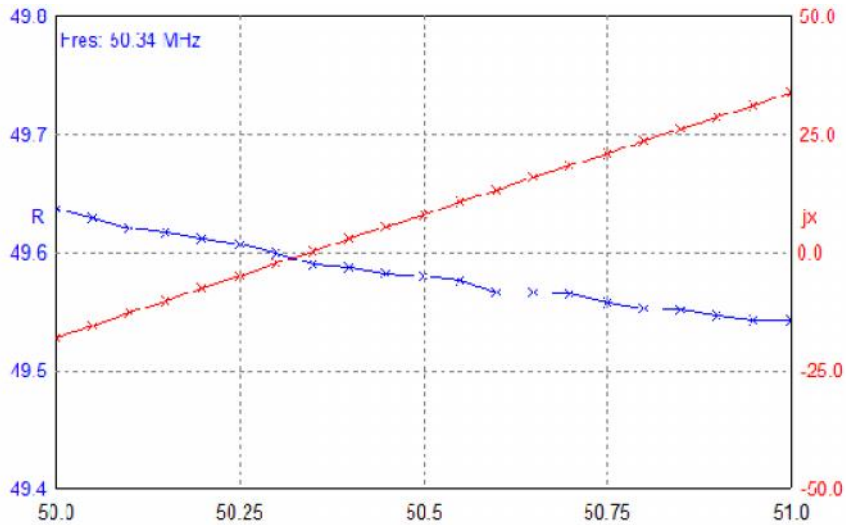
Figure 2 Z of the Pyradouble Antenna for the 50- MHz Band
