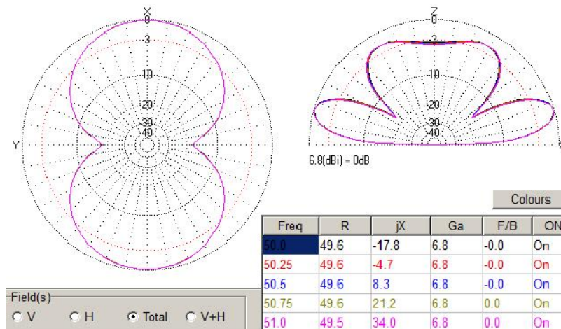
Figure 4 DD of the Pyradouble Antenna for the 50- MHz Band
