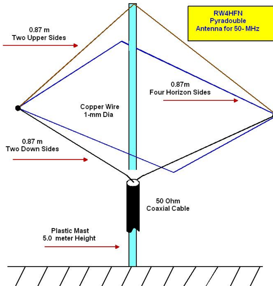
Figure 1 Pyradouble Antenna for the 50- MHz Band
