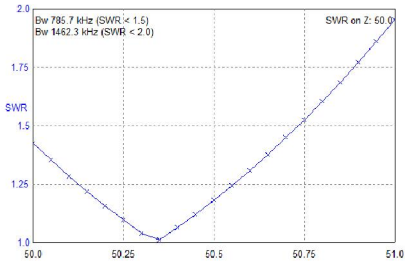
Figure 3 SWR of the Pyradouble Antenna for the 50- MHz
