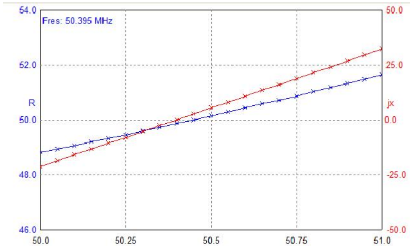
Figure 2 Z of the Pyramidon Antenna for the 50- MHz Band
