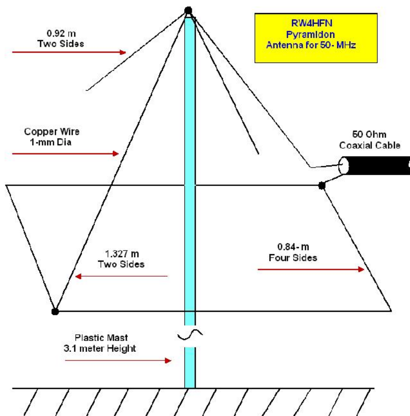
Figure 1 Pyramidon Antenna for the 50- MHz Band
