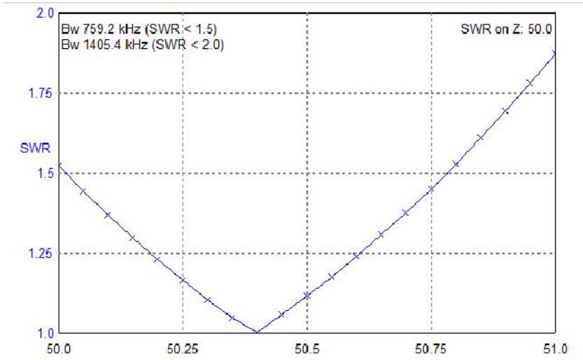
Figure 3 SWR of the Pyramidon Antenna for the 50- MHz
