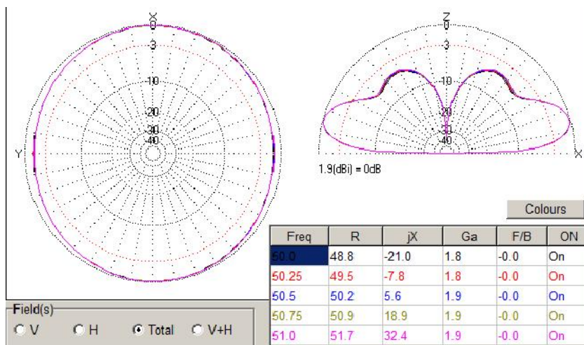
Figure 4 DD of the Pyramidon Antenna for the 50- MHz Band
